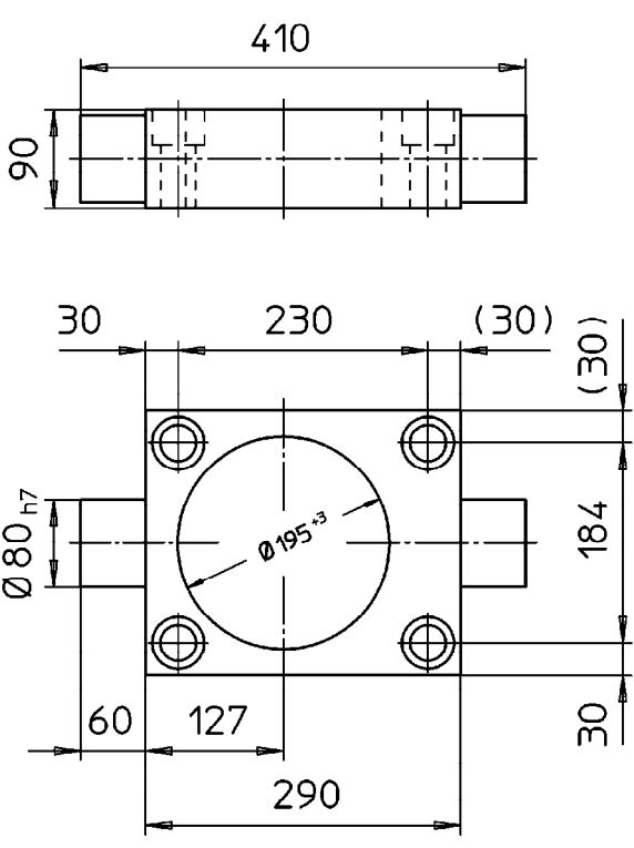
Kardan-Adapter
