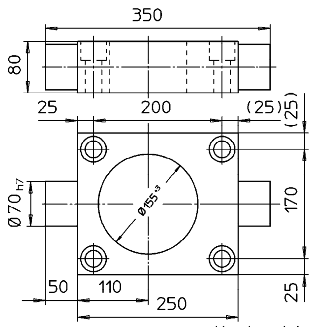
Kardan-Adapter
